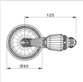
0R6241.B00.** Door handle on roses with exclusive Swarovski crystal
