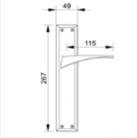
0A4752.000.** Door handle on plate
