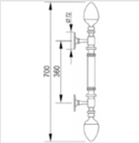
Set - 0N4483.000.** Individual sale - 0N4482.000.** Door pull handle on roses
