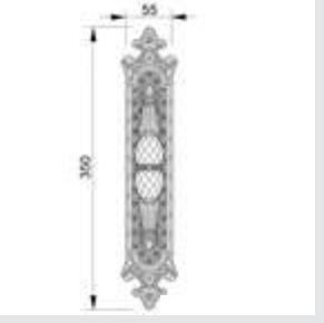
0M4605.S00.** 0M4605.SN0.** Door pull handle on plate with Swarovski crystal - Individual sale -
