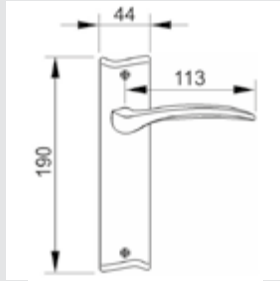
0A2251.000.** Door handle on plate
