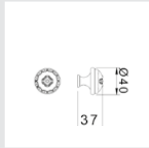
Ø 40mm - 0ZZ404.000.** Ø 33mm - 0ZZ403.000.** Furniture knob - Individual sale - Fixing screw Ø 4mm. Recommended Ø 4,5mm hole
