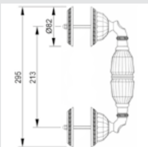
0N6204.000.** Door pull handle on roses with exclusive Swarovski crystal
