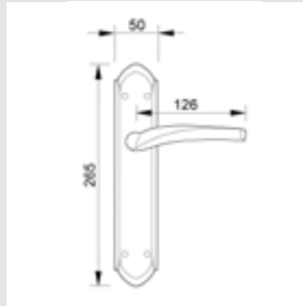
0A1353.000.** Door handle on plate
