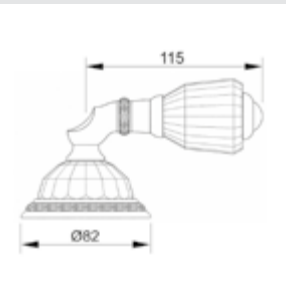
0R6263.000.** Door handle on roses with exclusive Swarovski crystal
