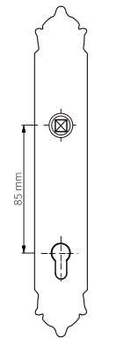
85Y EUROPROFILE KEY HOLE
