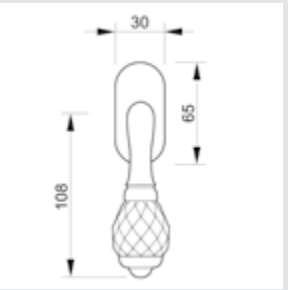
0V0740.000.** 0V0740.N00.** Applicable for right and left opening/hand. Window handle with Swarovski crystal - Individual sale
