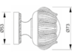
OC6538.000.** Door fixed knob
