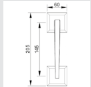
0N6403.000.** Door pull handle on roses - Individual sale -
