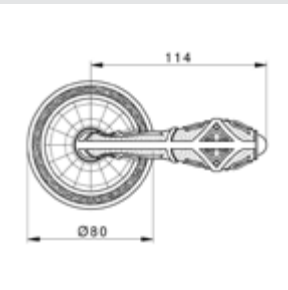
0R6234.000.** Door handle on roses with exclusive Swarovski crystal
