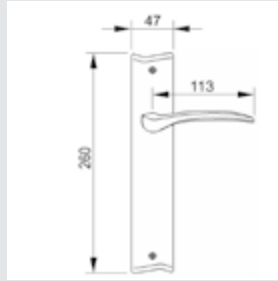
0A2351.000.** Door handle on large plate
