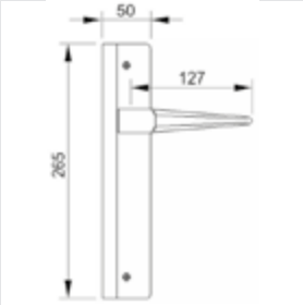
0A2754.000.** Door handle on plate
