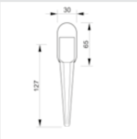
0V0754.000.** Window handle - Individual sale
