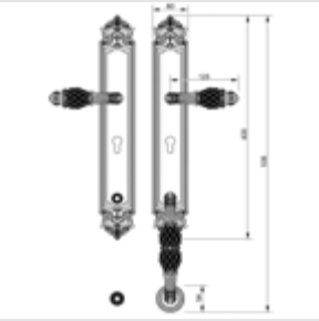
0J3705.S85Y.** 0J3705.SN85Y.** Entrance door set with keyhole europrofile 85mm
