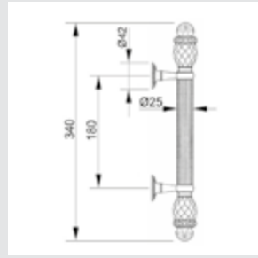
Set - 0N4765.000.** Individual sale - 0N4764.000.** Door pull handle on roses
