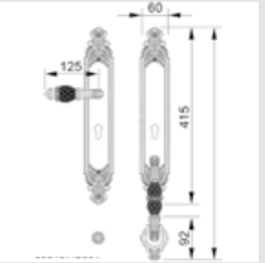
0J3407.S85Y.** 0J3407.SN85Y.** Entrance door set with keyhole europrofile 85mm with Swarovski crystal
