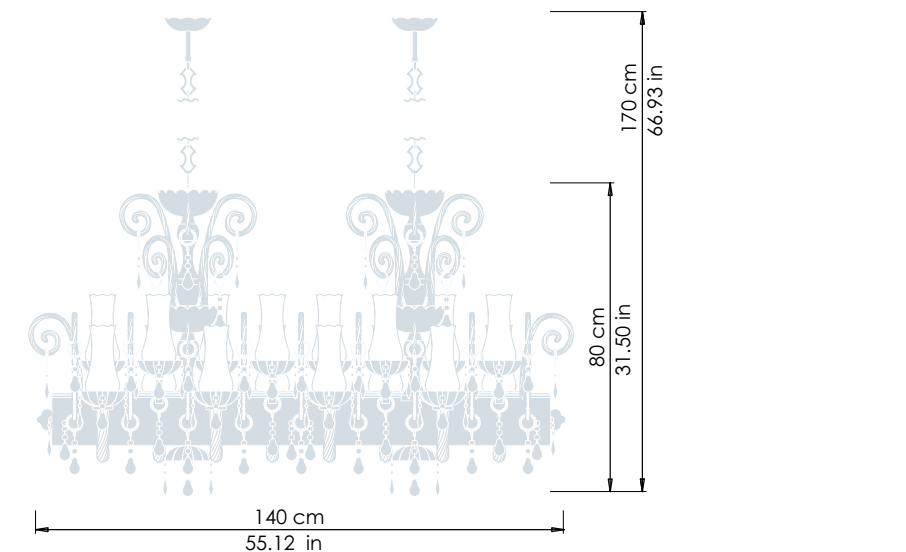
Art. 1315/16 lights L cm 140x90 / H cm 80-170 L 55.12x35.43 in / H 31.50-66.93 in
